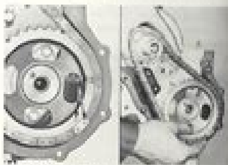
Fig. 2-100 Installing Timing Sprockets
