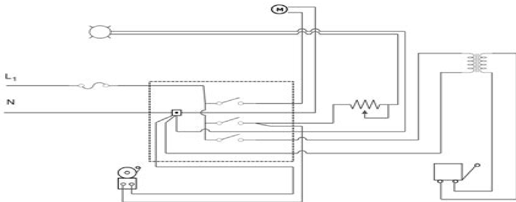
WIRING DIAGRAM
