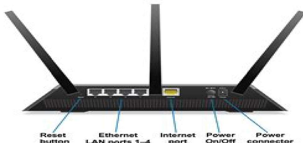
Figure 3. Router rear panel
