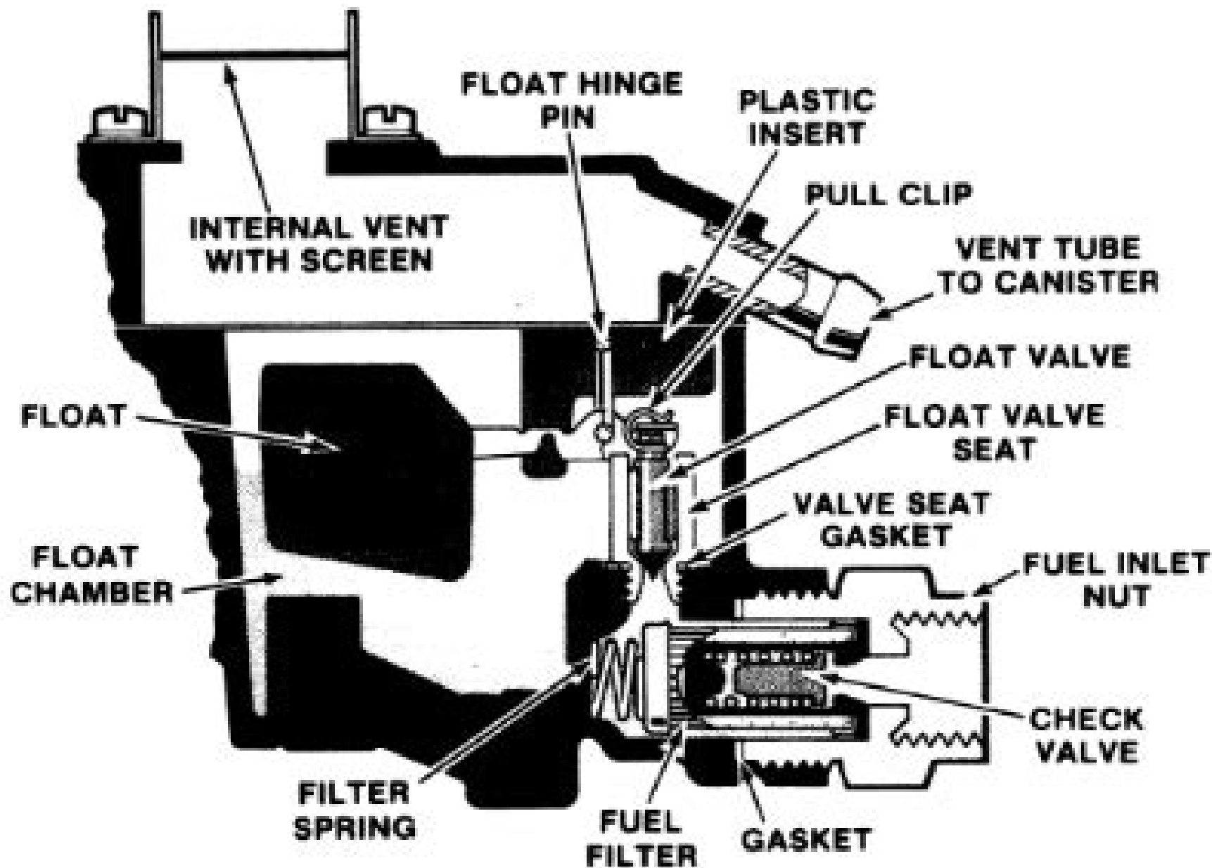
FLOAT SYSTEM
