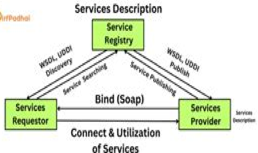
Fig. 1.4 Web Services Architecture cloud computing
