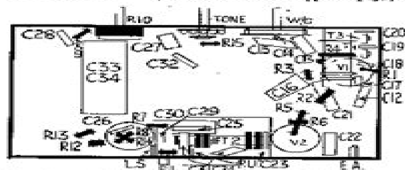
Layout diagrams of the MP chassis (condensable on right) identifying components. Condensers are in outline and resistors in solid black to aid reference.
