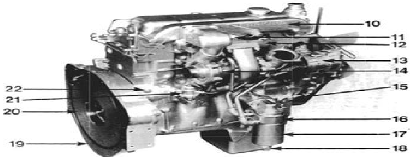
VIEW OF CAMSHAFT SIDE OF T4.236 ENGINE
