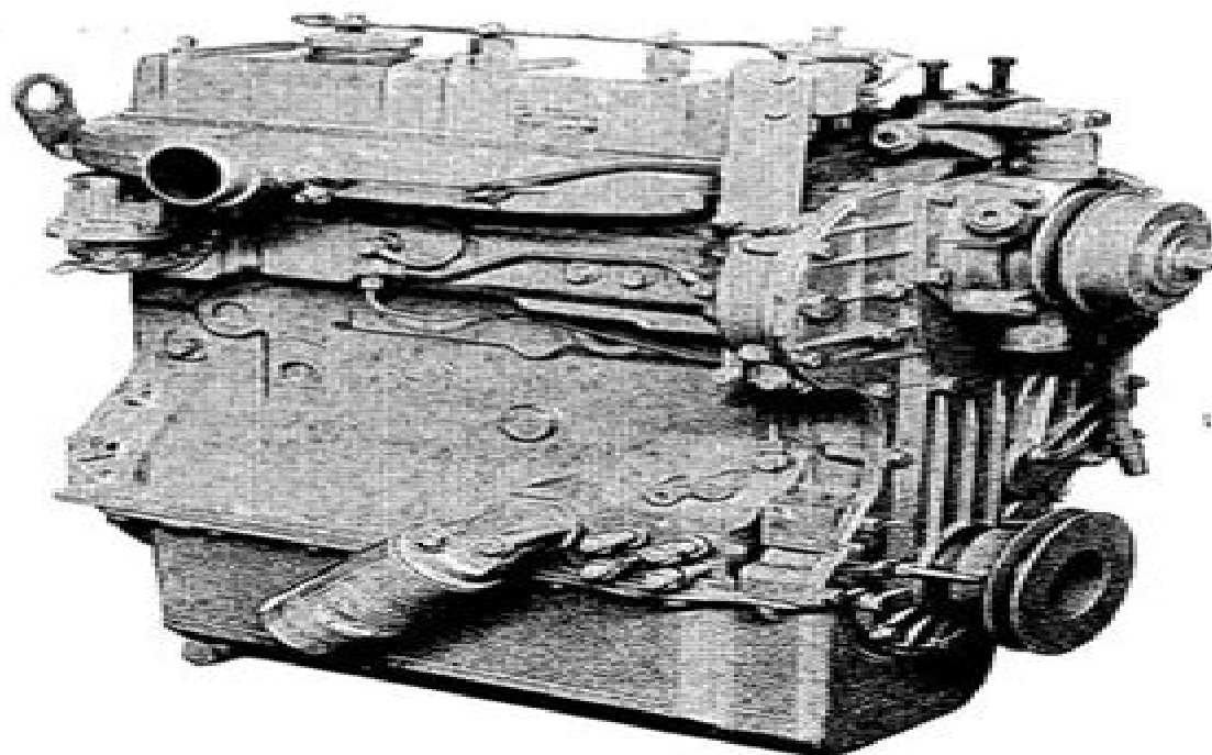
View of Front Right Hand Side of Engine.
