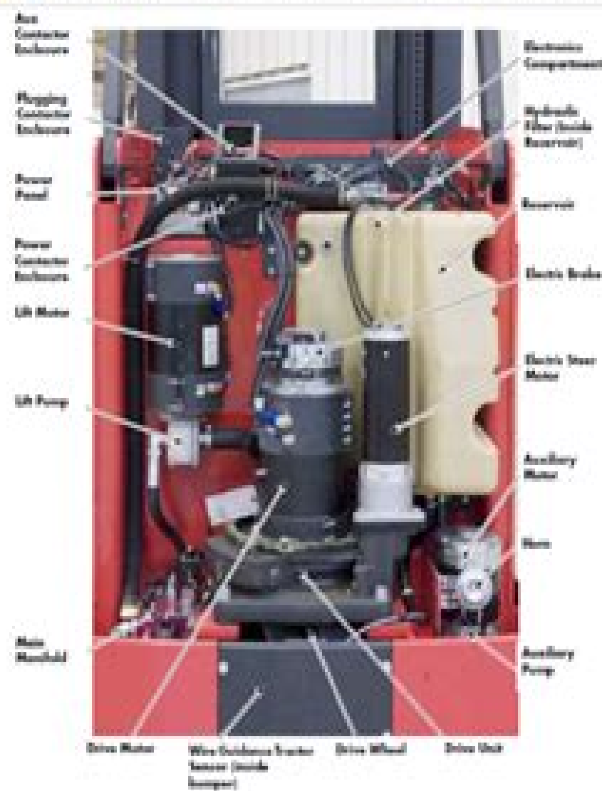
Figure 2-2 Hydraulic Components
