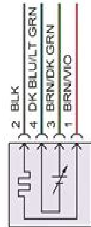
OXYGEN SENSOR 2/1
