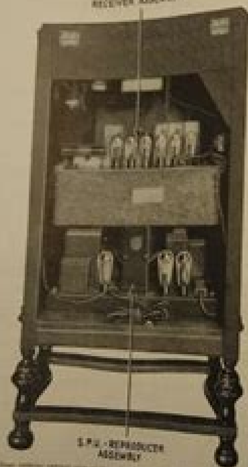
RECEIVER ASSEMBLY
