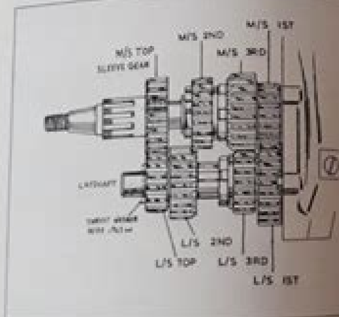
Illustration 9-15 - Gear cluster seen from the rear
