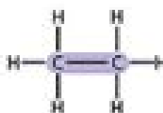
Single bond
