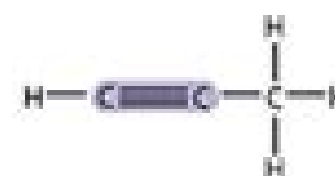
Triple bond
