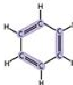
Double bond
