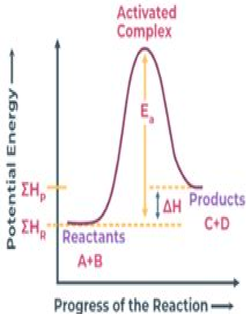
Endothermic Reaction
