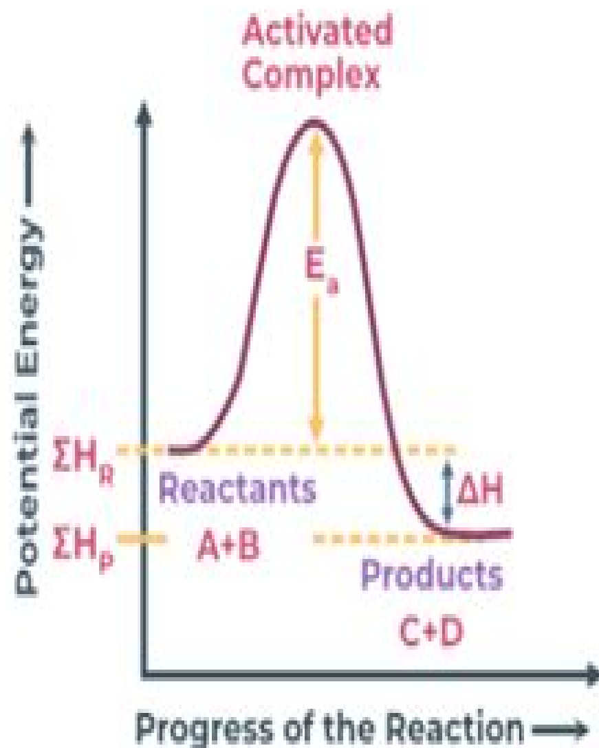
Exothermic Reaction
