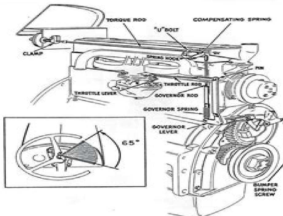
Fig. 46 Governor Linkage
