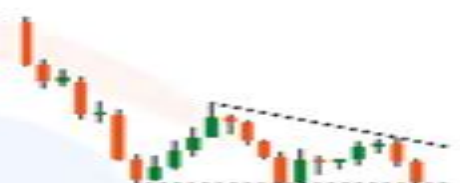
DESCENDING TRIANGLE
