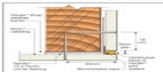
FIGURE 16 SEALANT FILL OPTION
