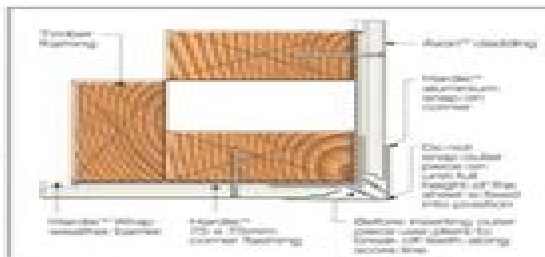
FIGURE 17 SNAP ON CORNER OPTION
