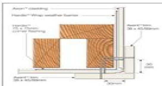
FIGURE 18 TRIM CORNER OPTION
