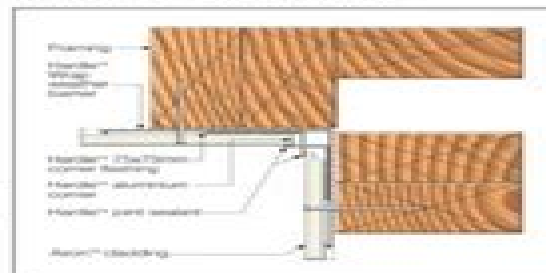
FIGURE 20B ALUMINUM INTERNAL CORNER
