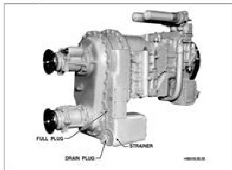
Figure 11. 5000, 6000 Series Models With Dropbox – Full Plug Location
