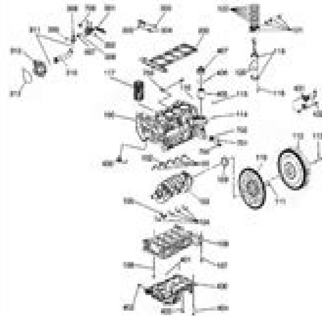
Fig. 21: View Of Engine Block & Components Courtesy of GENERAL MOTORS CORP.
