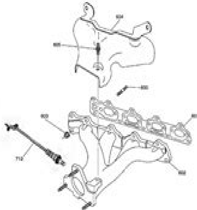
Fig. 20: View Of Exhaust Manifold & Components Courtesy of GENERAL MOTORS CORP.
