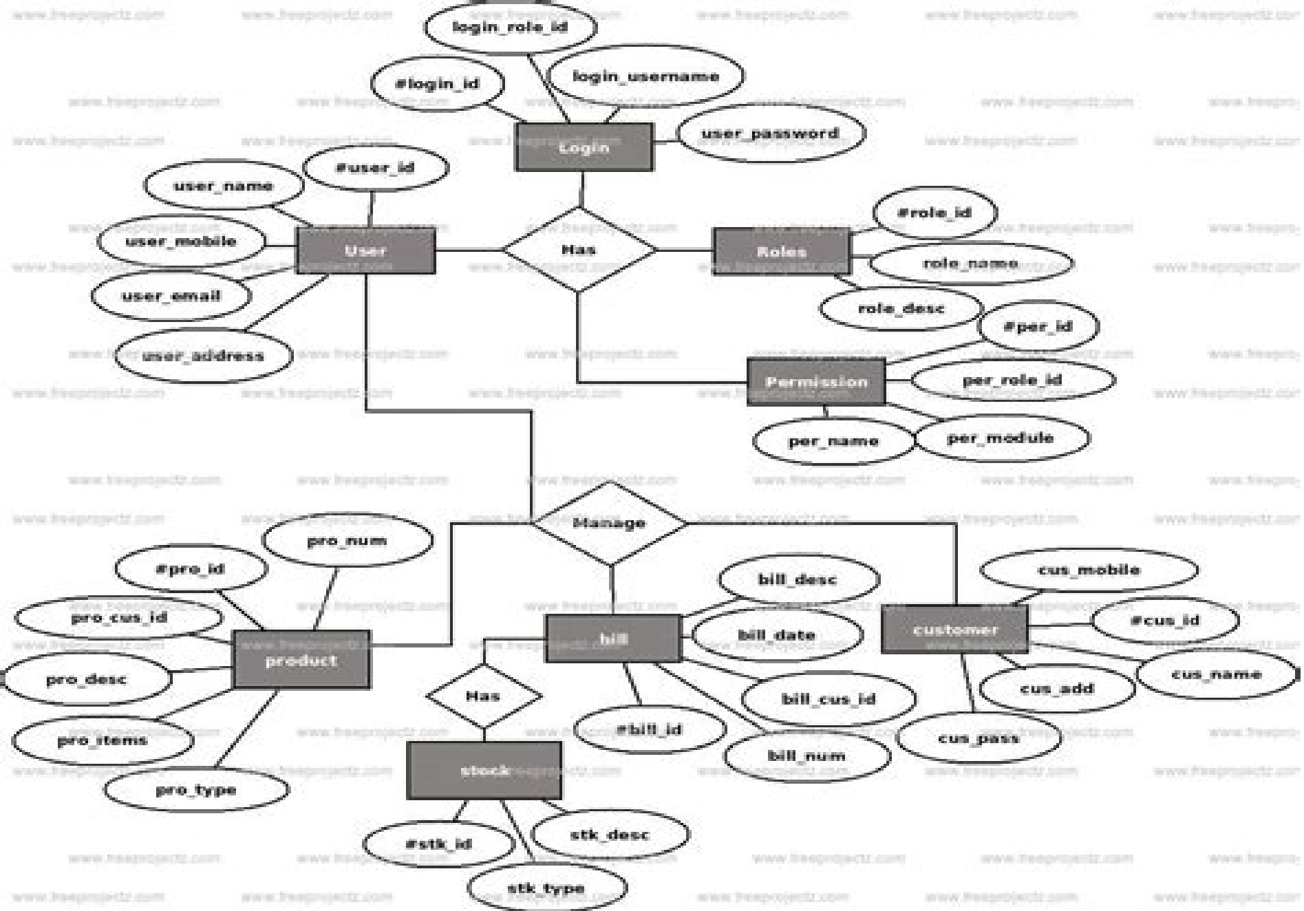
ER Diagram For Stock Management System
