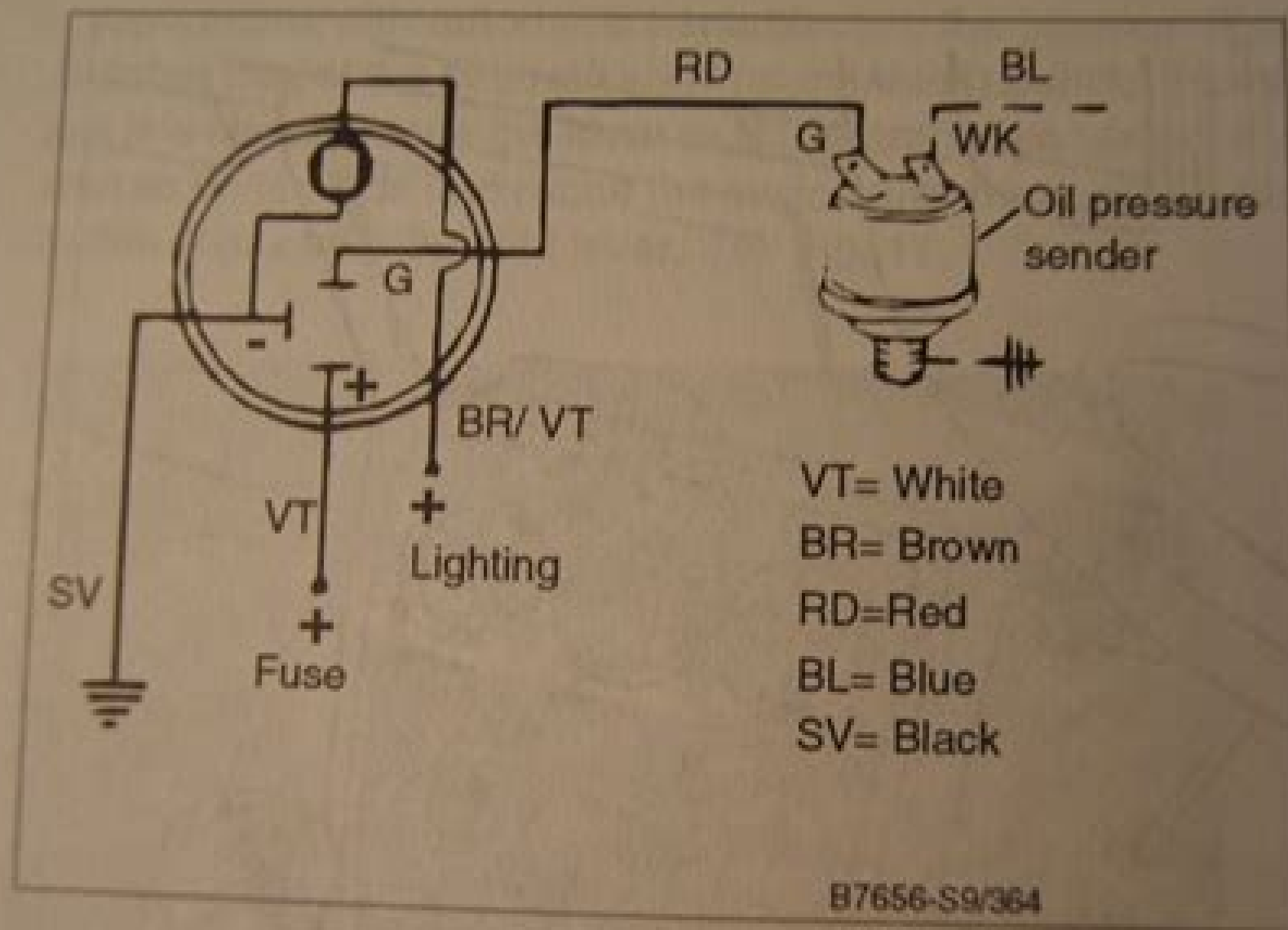
Fig. 19. Wiring diagram for extra oil pressure gauge.
