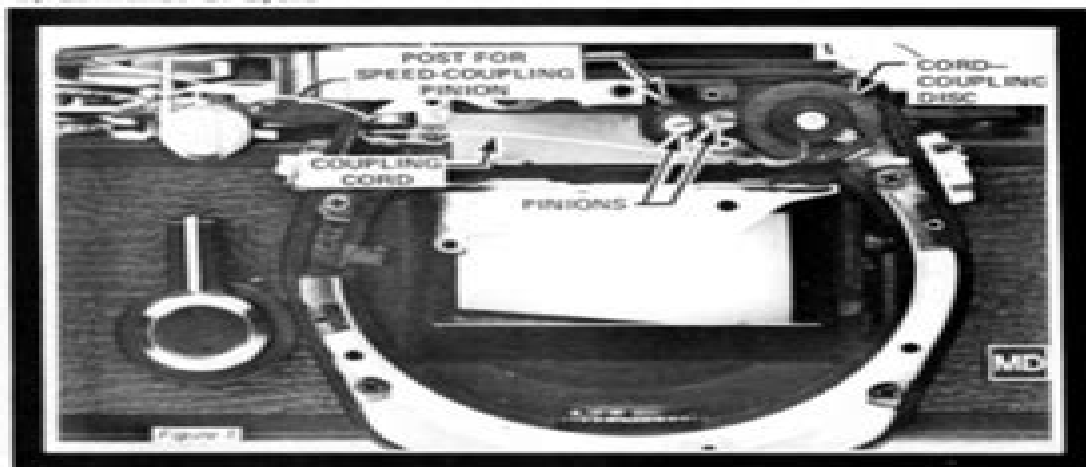
Front of the OM-1 "MD" after removing the speed-sensing and aperture-sensing rings. "MD" stands for "motor drive." A set of contacts at the bottom of the camera, next to the FP-sync contacts, signals the motor-drive accessory.
