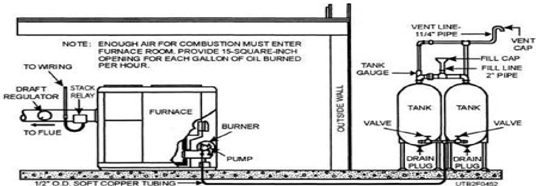
Figure 4-52.—Diagram of piping for inside or outside elevated tank installations.
