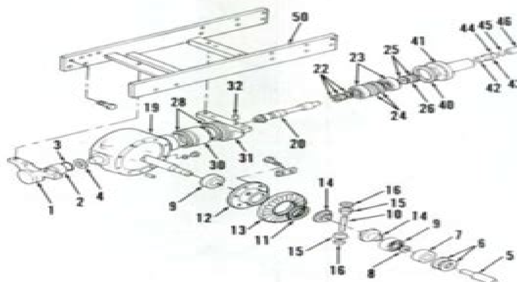
Fig. 18—Exploded view of front wheel drive differential assembly and bevel drive gears used on 1710 and 1810 models. Refer to Fig. 17 for legend except for those listed.
