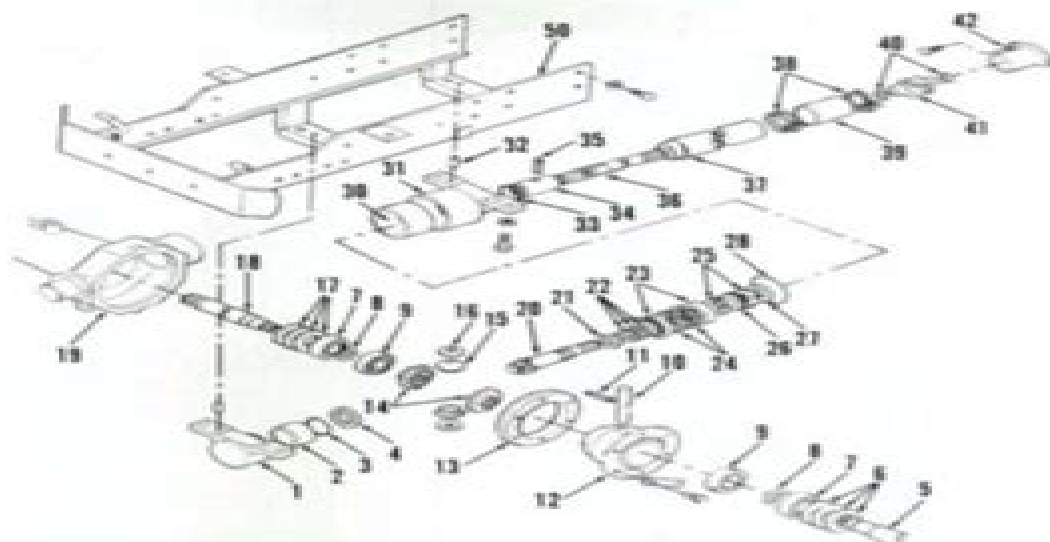
Fig. 17—Exploded view of front wheel drive differential assembly and bevel drive gears used on 1110 and 1210 models.
