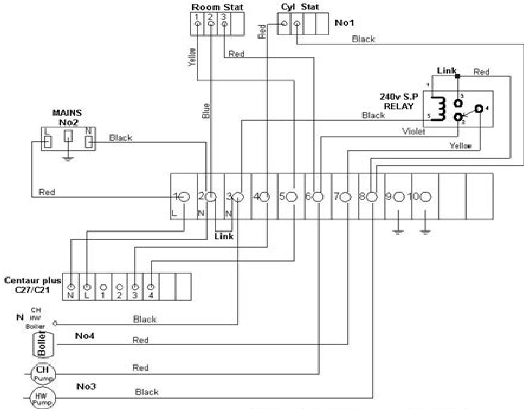
SMC Controller Twin Pump System
