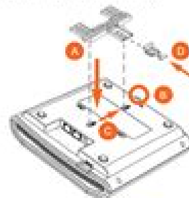
Figure 3. Attaching the T-bar bracket to the AP
