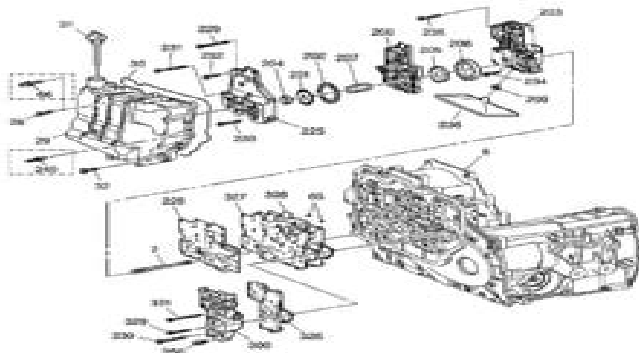
Fig. 2: Transmission Case and Associated Parts Disassembled View (2 of 3) Courtesy of GENERAL MOTORS CORP.
