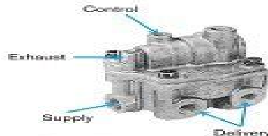
Figure 41. Bobtail proportioning relay valve.
