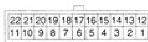
Wire End View of Connectors
