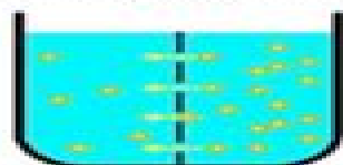
Diffusion (Solvent moves by concentration gradient)
