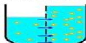
Osmosis (Water moves by concentration gradient)
