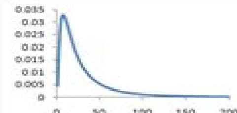
Log Normal Distribution
