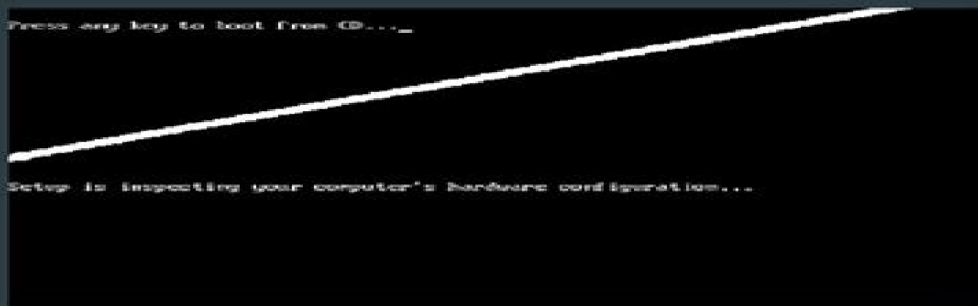
Figure 58.Boot from CD
