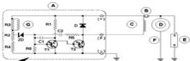
12V Control Unit Circuit Diagram
