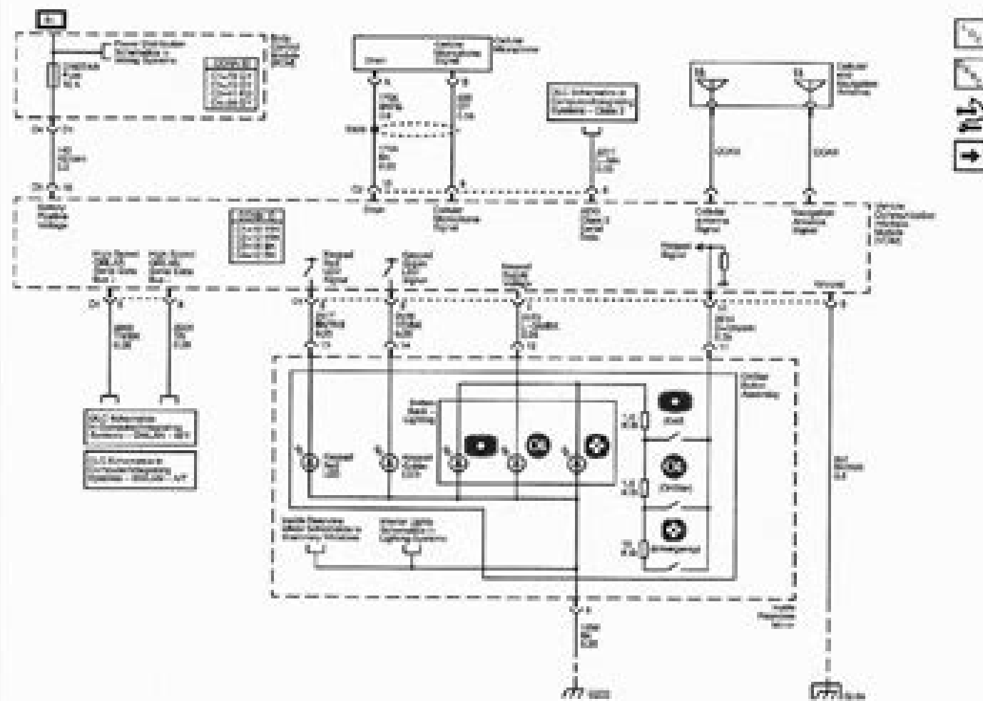
Fig. 9: Antenna, DLC, Ground, Power and User Inputs Schematic Courtesy of GENERAL MOTORS CORP.
