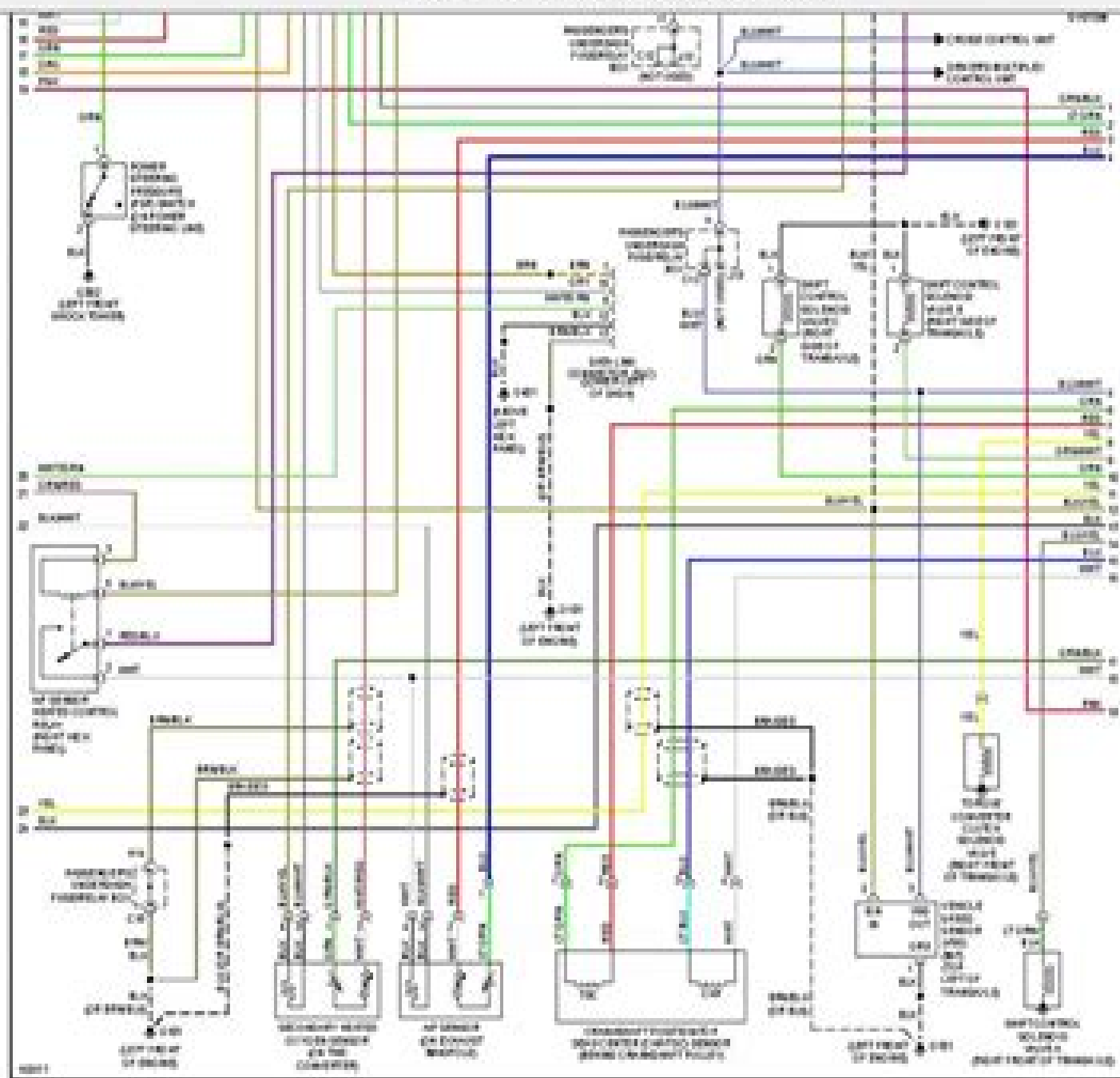
Fig. 28-2-2. Engine Performance Control, CVT (See List of Symbols) (2 of 2)
