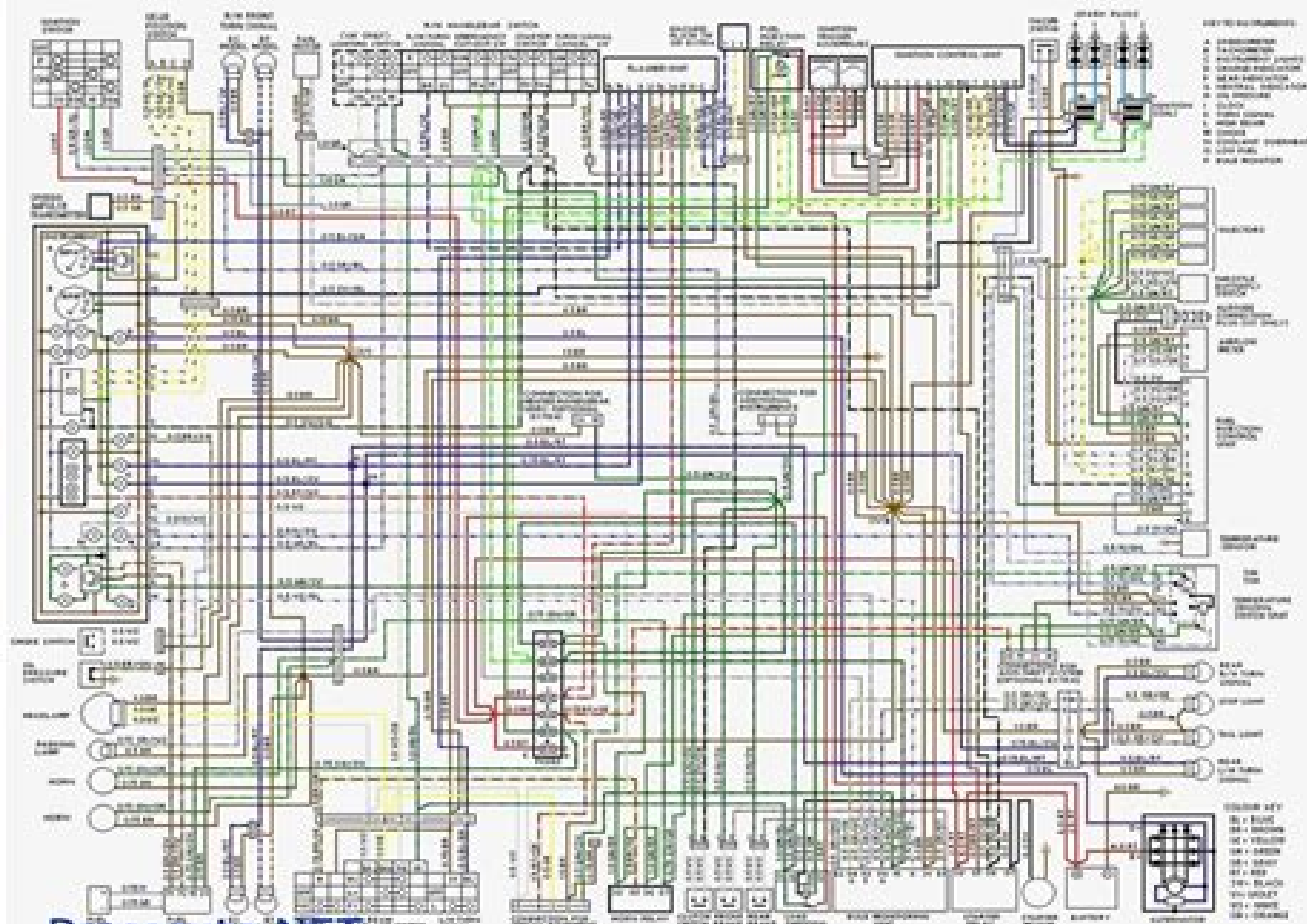
Wiring Diagram - early 1900 RS and RT model
