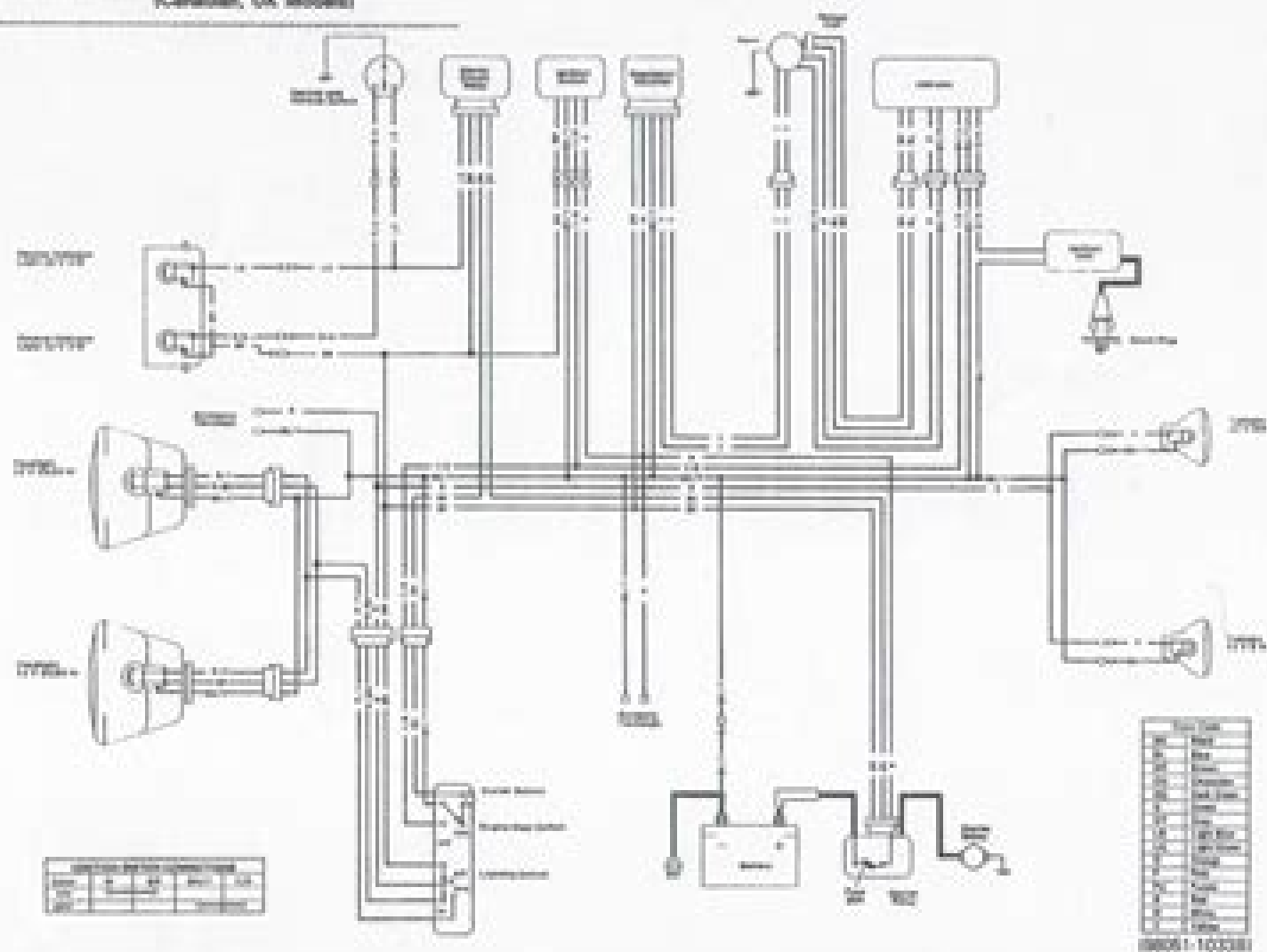
Wiring Diagram KLF220-A1, A2, A3 (All Models) KLF220-A4, A5, A6, A7, A8 (Canadian, UK Models)
