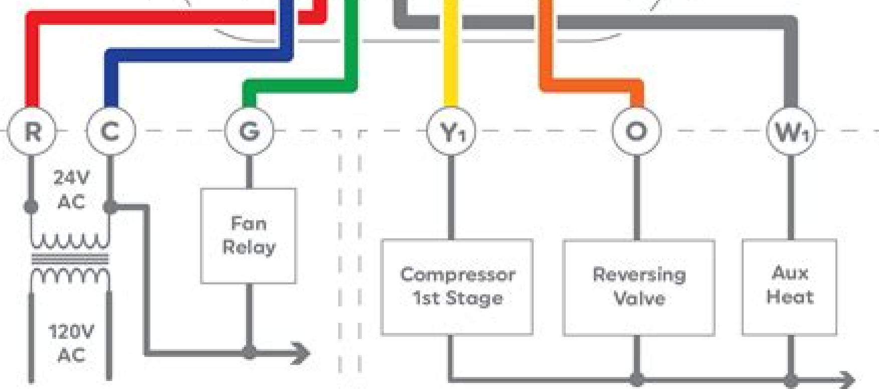
Heat Pump Connections
