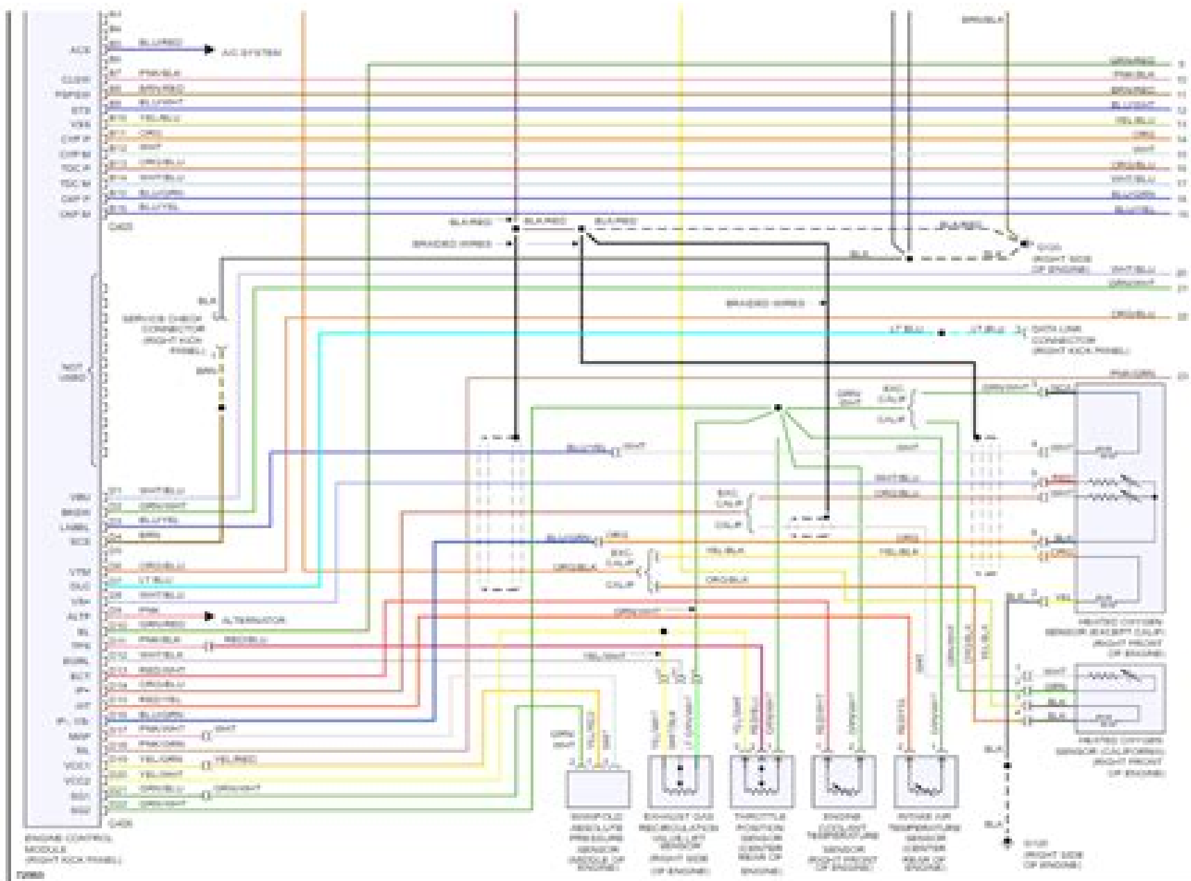
Fig 1: 1.5L VTEC, Engine Performance Circuits (1 of 2)
