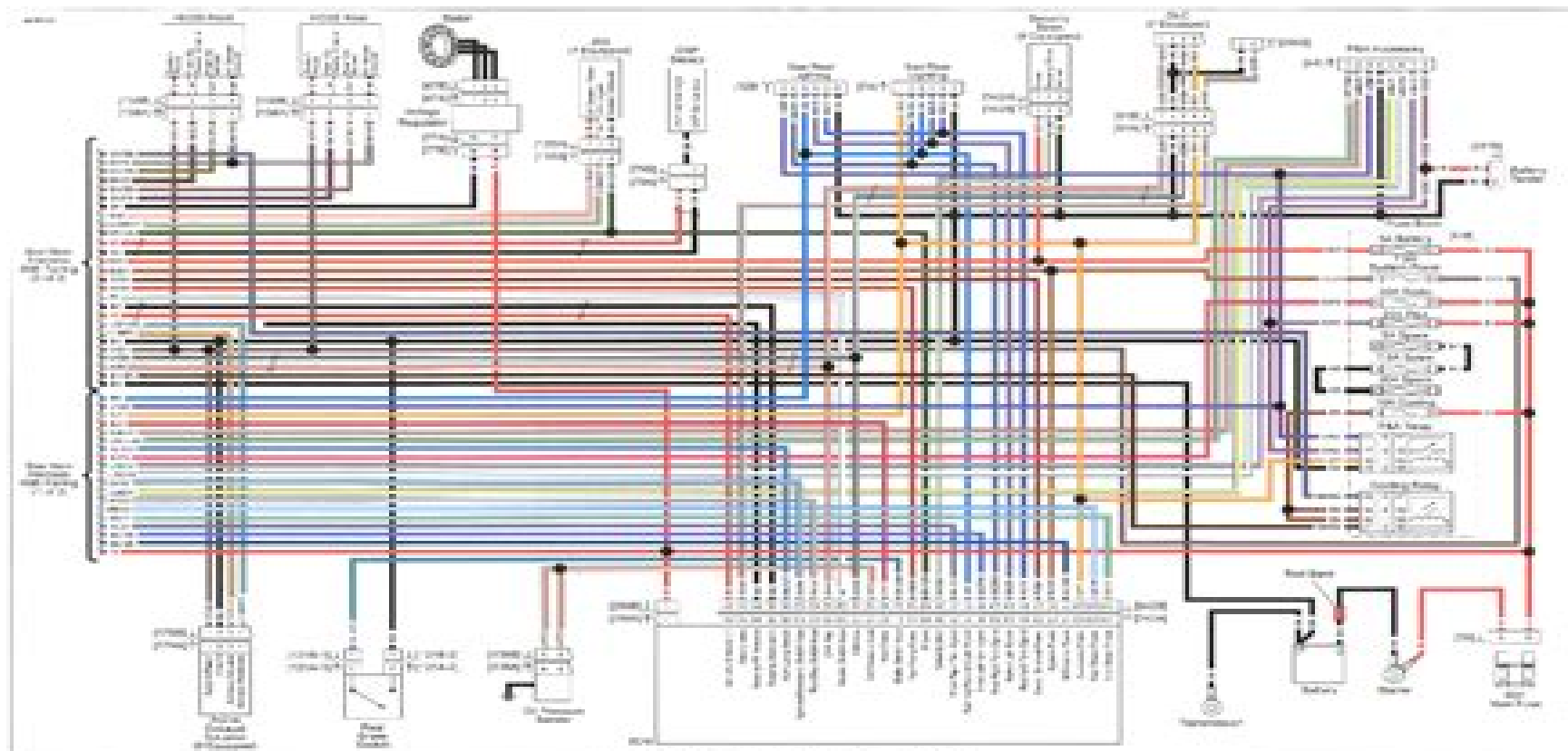
Figure 8-12 Main Harness (2 of 2) (3rd Year) (After Parking)
