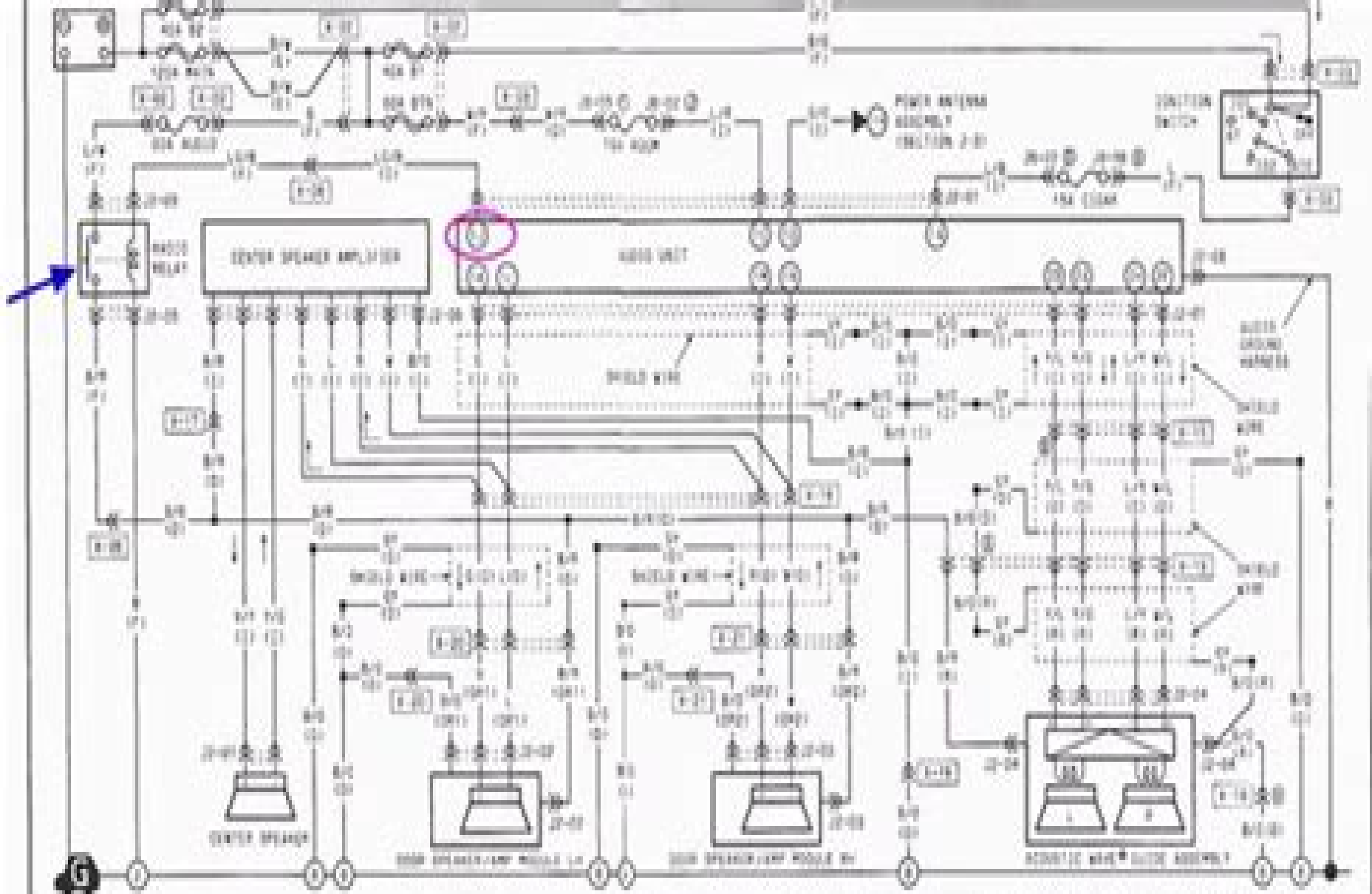
20-01 RADIO UNIT (1)
