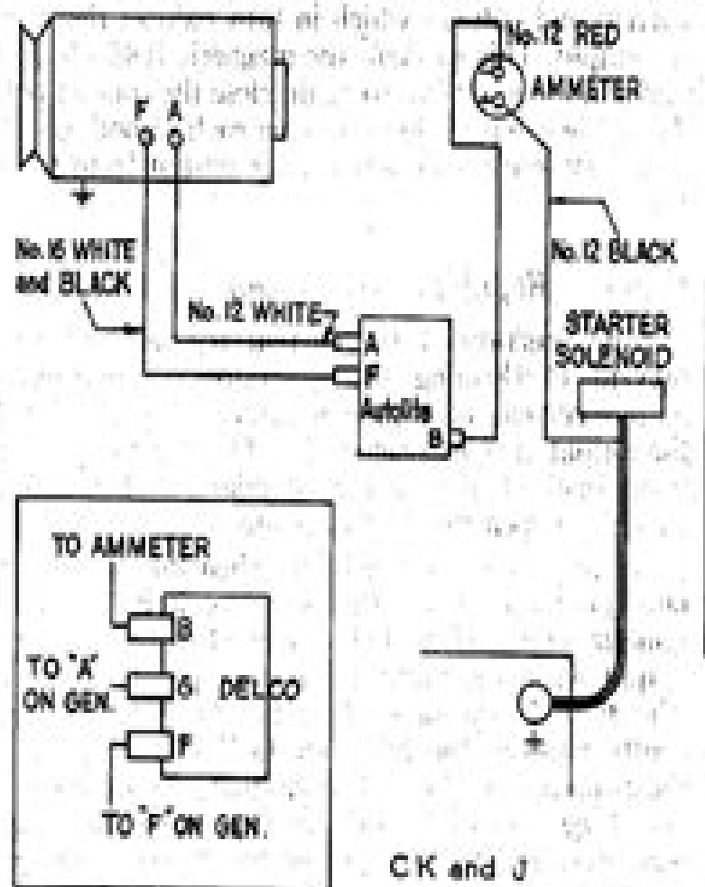
GENERATOR CIRCUIT
