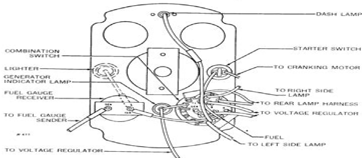
Instrument Panel Wiring
