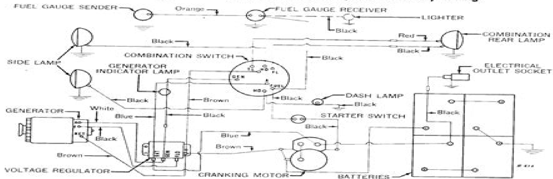
Instrument Panel Wiring
