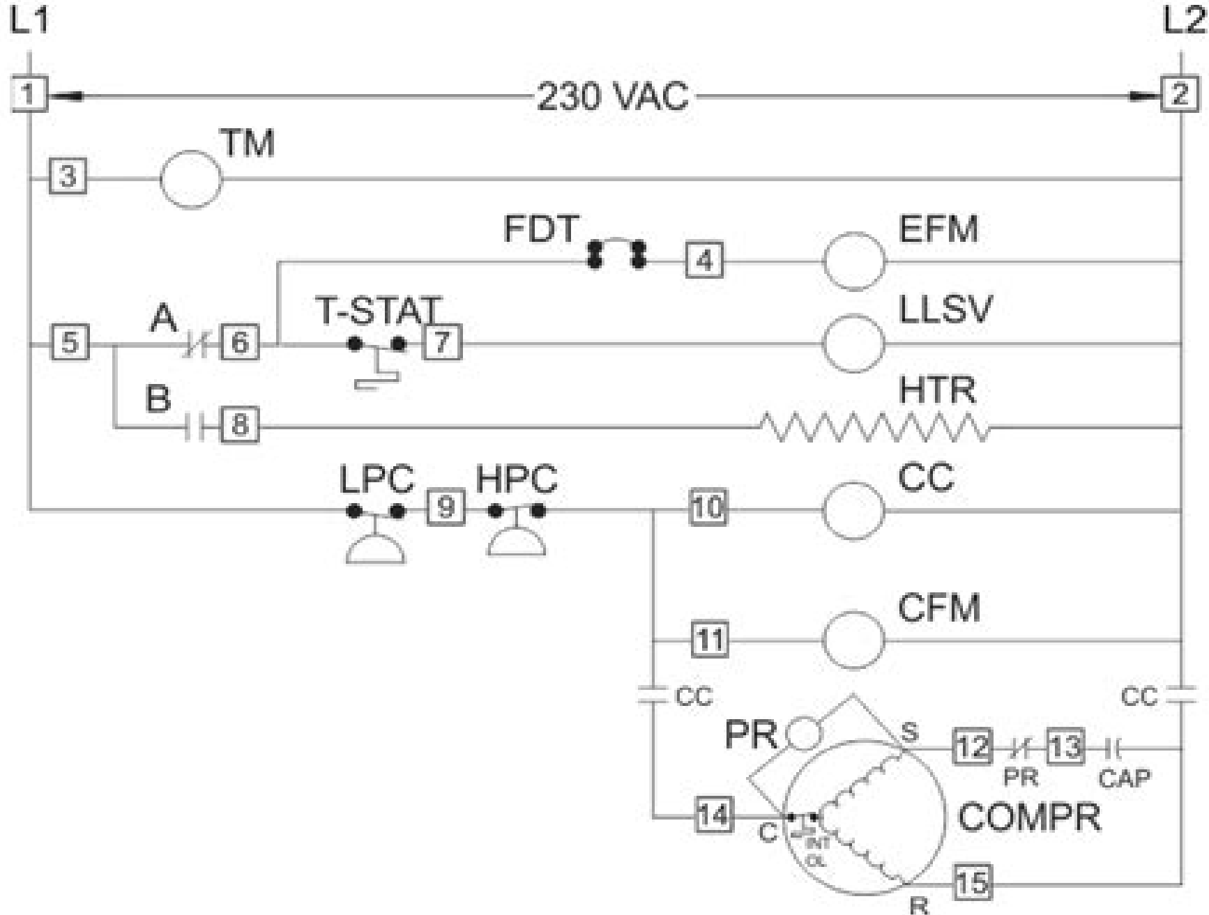
Walk-in Freezer with Electric Defrost
