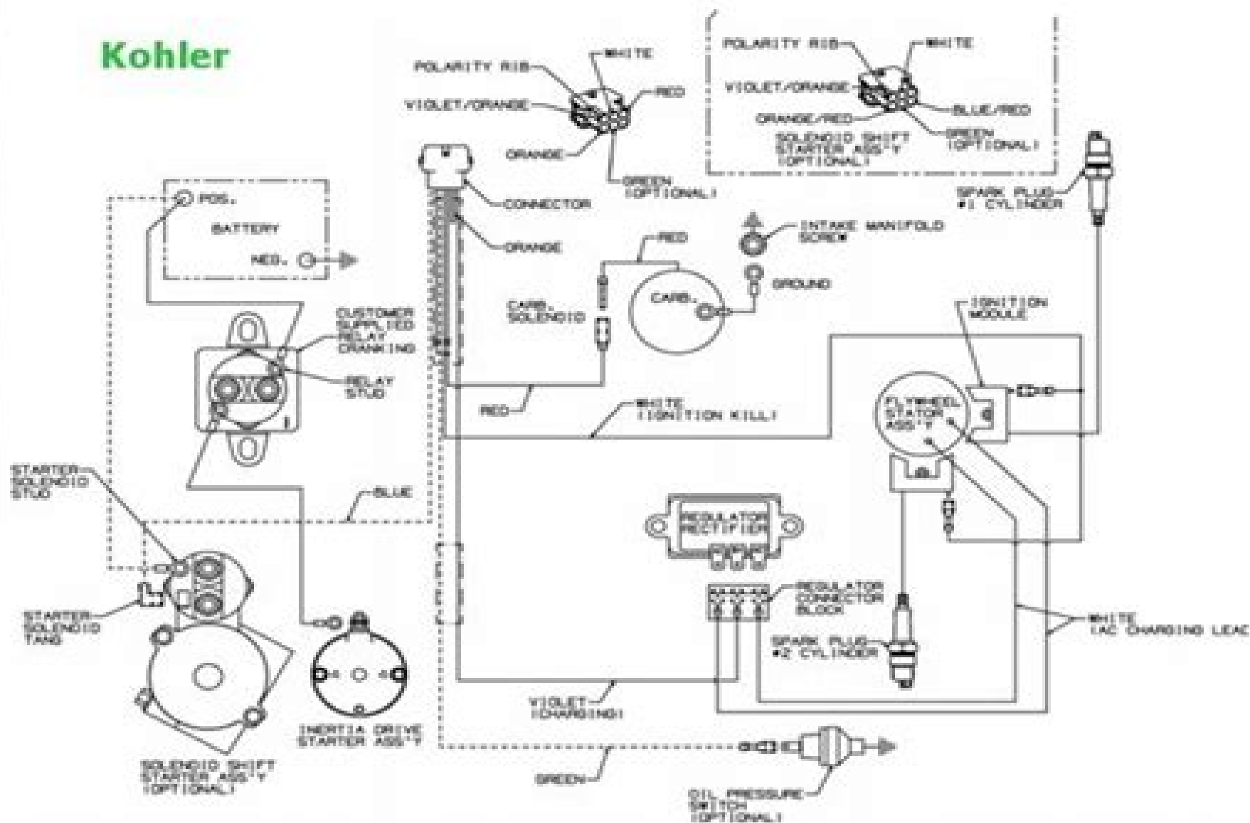
Figure 2-16. Wiring Diagram - Fixed Timing Ignition System.
