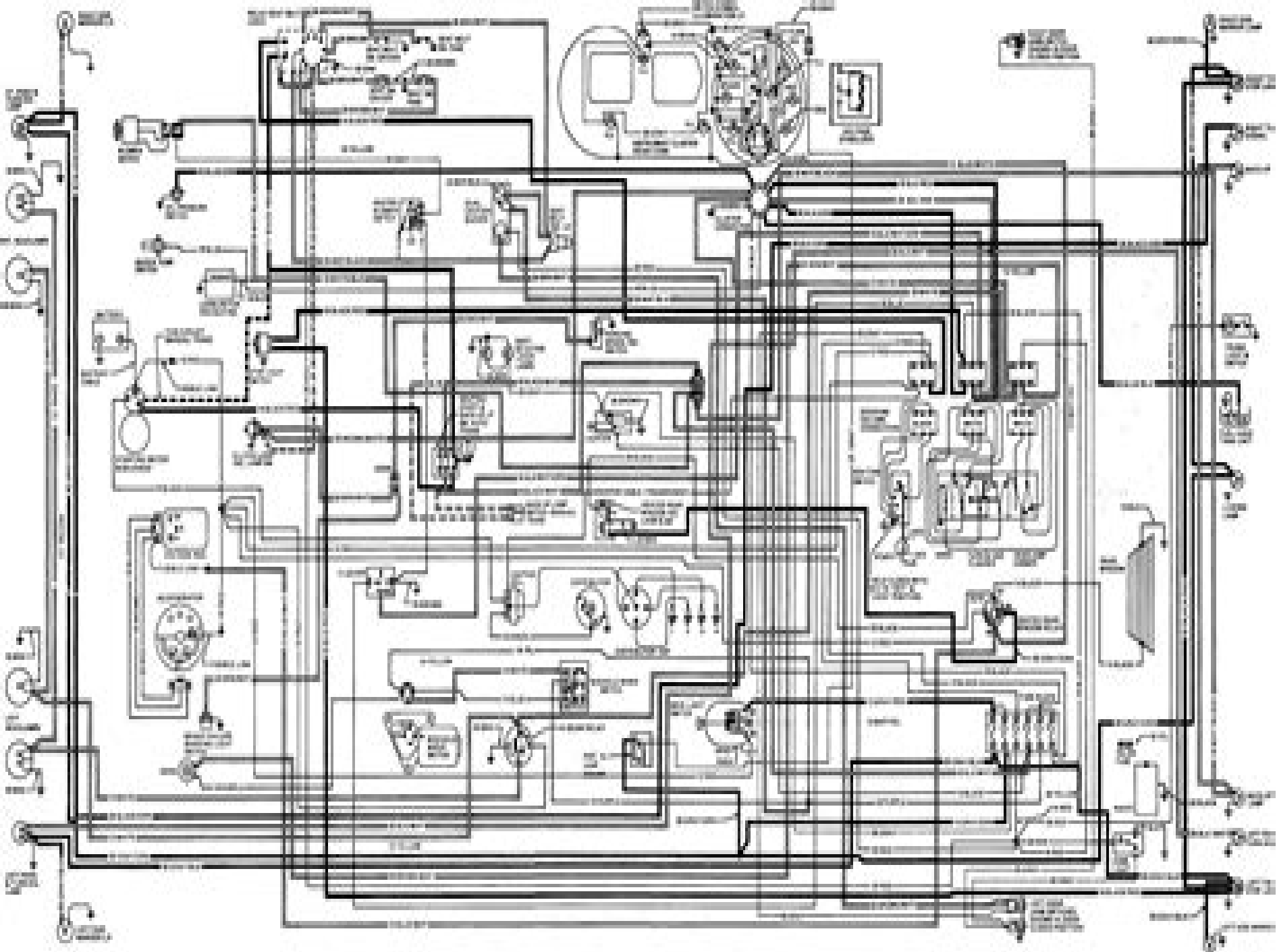
Figure 14-12 Fuel System Wiring Diagram
