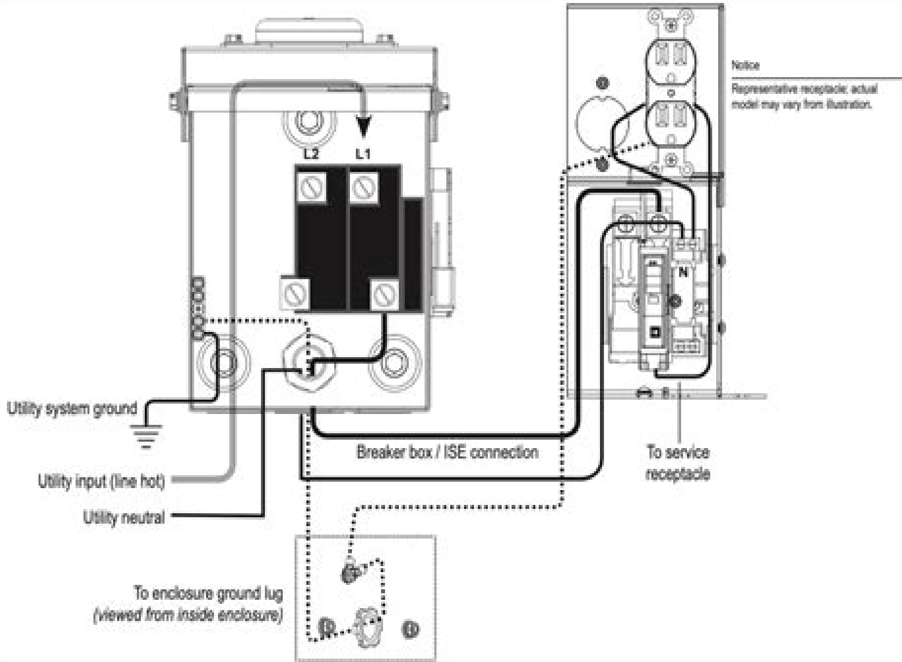
Simplified wiring diagram
