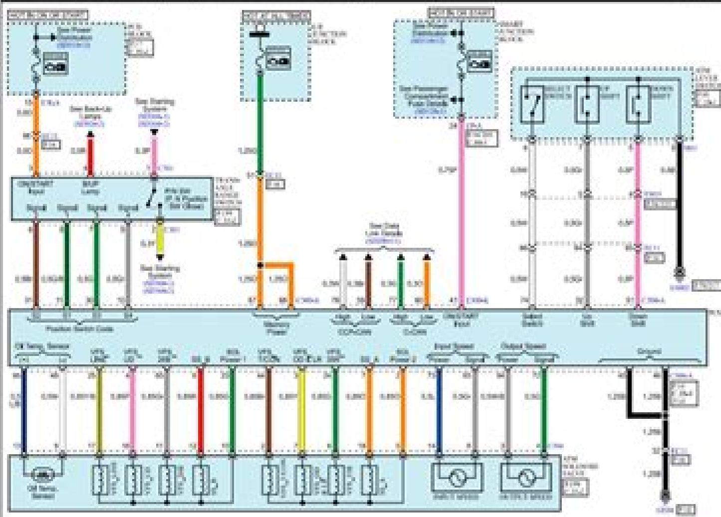
Automatic Transaxle Control System (G400 - LAMBDA II 3.3L MPI) (1)
