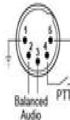
C 0379 5 Pin XLR Wiring Diagram
