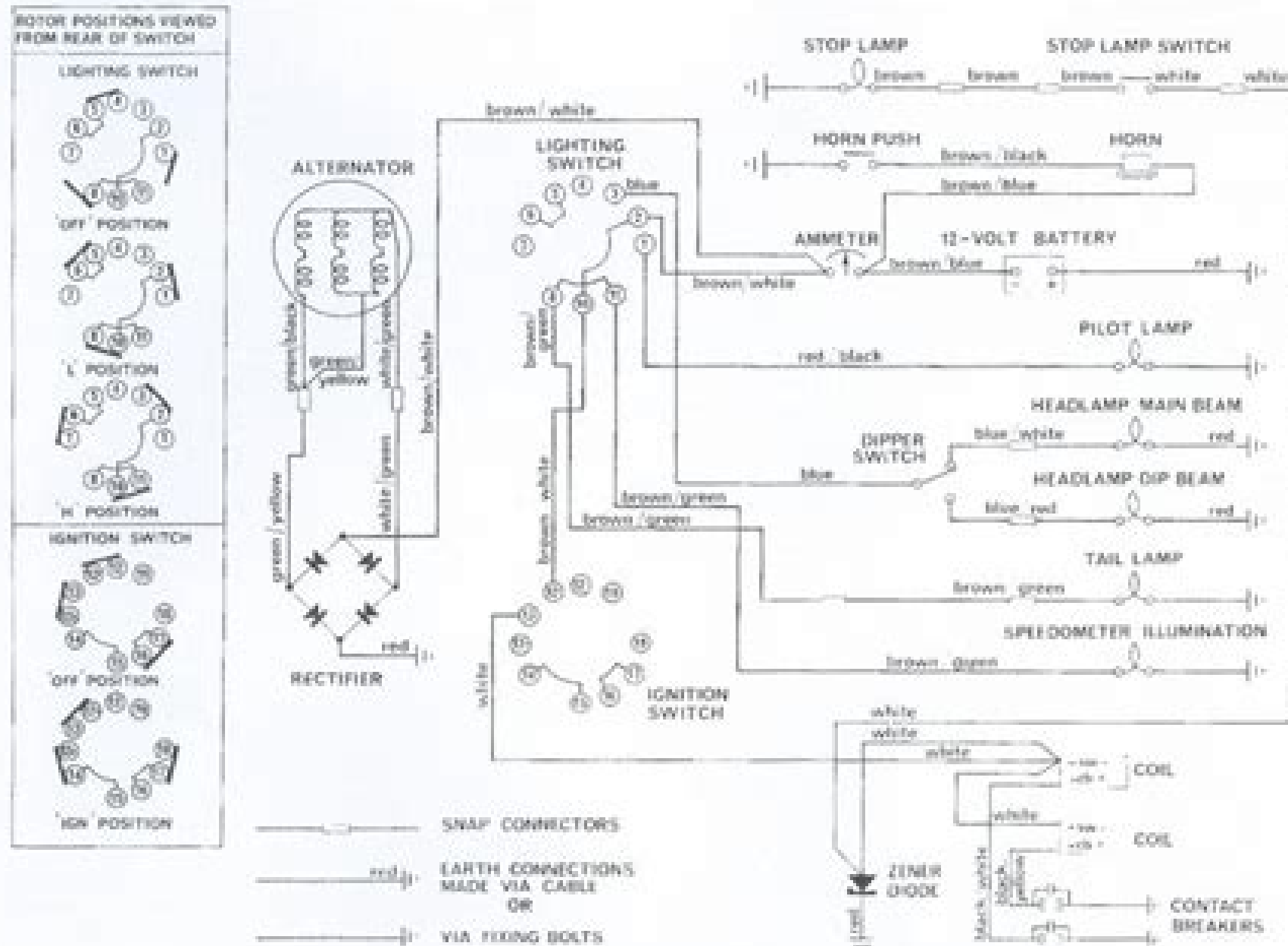
Fig. H34. Wiring diagram—Coil ignition 12 volt models with nacelle from engine number DU2MPS
